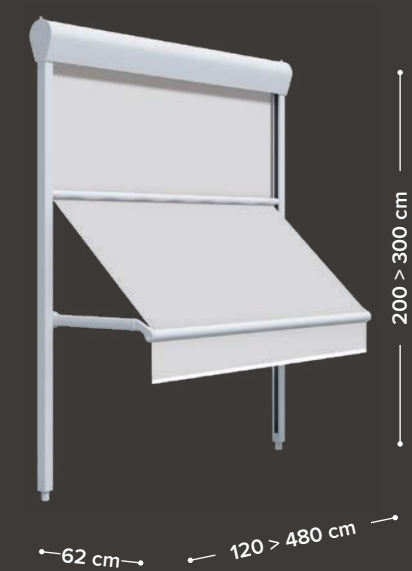
DIM 6 with cassette / con cofre
